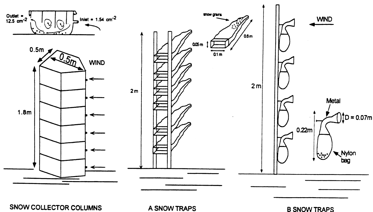
Fig. 1. The drifting-snow gauges.
