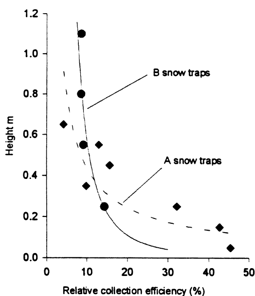
Fig. 5. Relation of the collection efficiency, relative to the snow-collector columns, with heights for the type A and B snow-trap gauges. Lines are fitted to the data (see Table 1).
