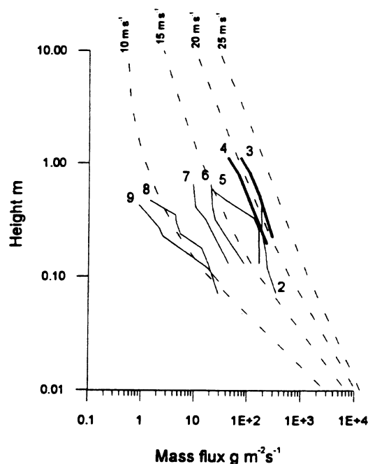
Fig. 7. Experimental mass-flux profiles vs height obtained at La Molina. The values of the A (profiles 2, 5, 6, 7, 8 and 9) and B (profiles 3 and 4) traps have been corrected applying the collection efficiency rates obtained from the comparison with the snow-collector columns. Dashed lines represent the theoretical values proposed by Mellor and Fellers (1986) (see Table 2).
